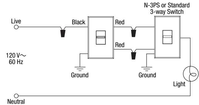
Figure 2. 3-Way Wiring
