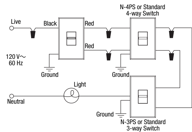
Figure 3. 4-Way Wiring
