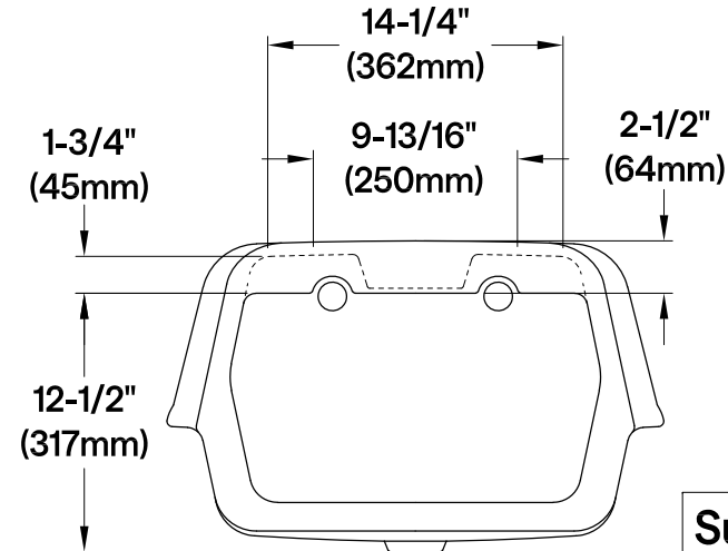
Sink Back View
