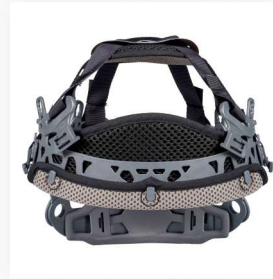
Flexible 6-Point Suspension System Open-frame design enhances airflow, stability, and fit
