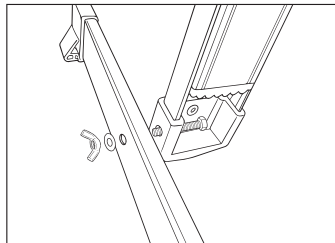
stabilizing bar
