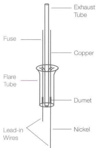
Figure 1- Mount parts assembled
