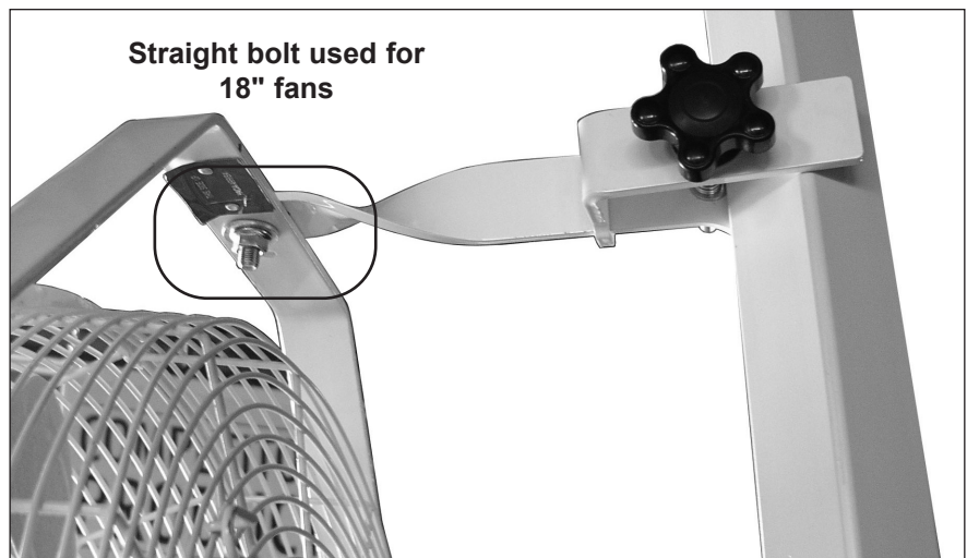
L-bolt used for fans that have an eyebolt
