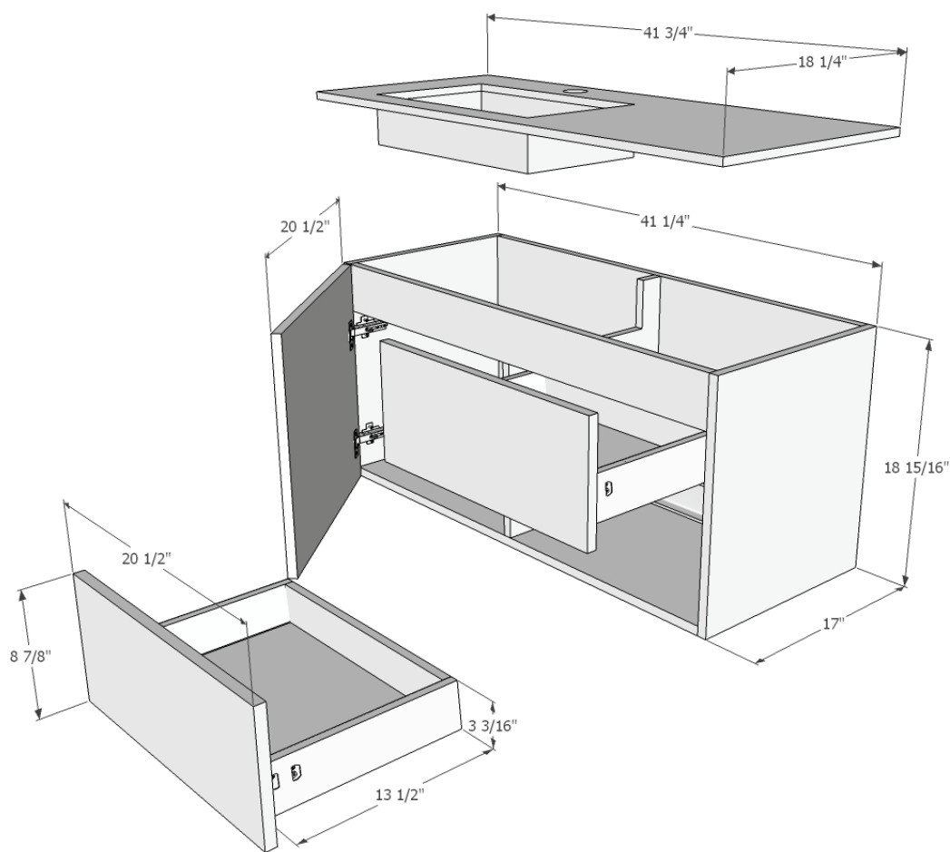
SINK DETAIL
