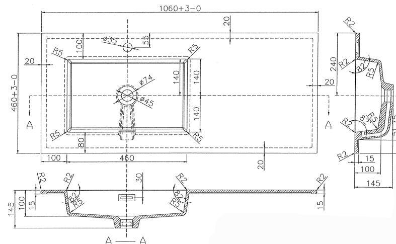
SINK DETAIL
