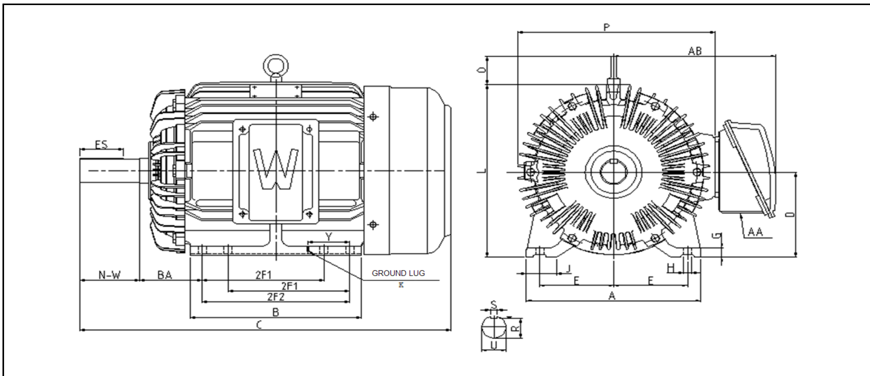
DIMENSIONS - INCHES
