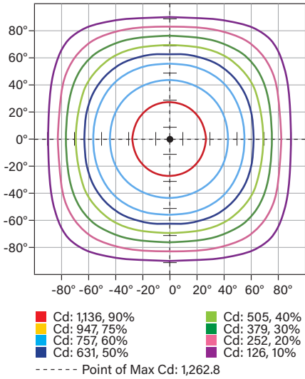
ISOCANDELA PLOT
