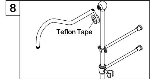
8. Apply Teflon tape on the shower arm threads then secure one end to the add on shower.
