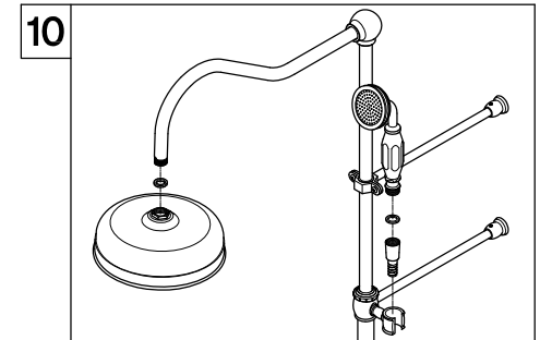
10. Tighten showerhead to shower arm and hand shower to the hose.
