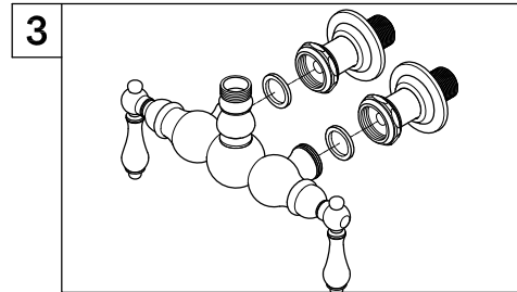
3. Before mounting the faucet onto supply elbows, apply small black washers onto both water inlets of faucet.
