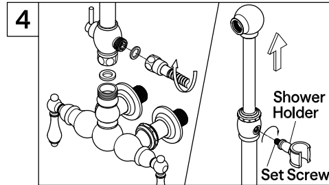
4. Install 60" shower riser onto faucet body. Remove the shower holder and the set screw inside. Pull up the upper tube from the riser body and adjust the upper tube to its appropriate height. Install the shower holder and set screw back onto the riser body. Make sure the set screw not over tightened, otherwise it will push aside the upper tube and cause water leakage.
