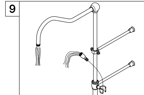
9. Turn on the faucet and let hot and cold water to run for at least one minutes to clean any debris inside the water line.
