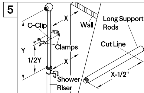
5. Install the c-clip and clamps on the upper tube at the "1/2Y" location. Adjust and keep the shower riser in a plumb direction, then measure the wall installation space "X" for deciding to use short or long support rod. If cutting long support rod is needed, you should cut it to fit as long as "X"-1/2 inch.
