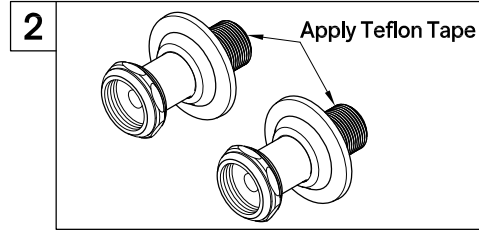
2. Apply Teflon tape on the threads of the copper shank. Install the elbow.
