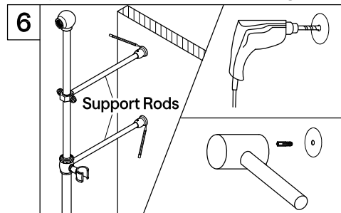
6. Place a base onto the wall and trace around it with a pencil. Drill holes at the marked locations and insert anchors into the holes with a hammer until flush with the wall.
