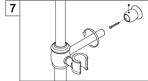
7. Screw the base to the wall with the mounting screws. Place the unit, with the small hole in the base underneath, over the mounting plate by tightening the screw with screwdriver until the base is tightly fixed.
