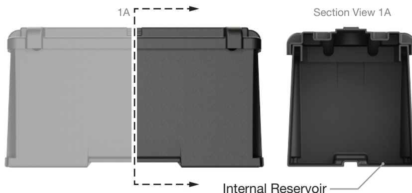
Lock-Down Knob
