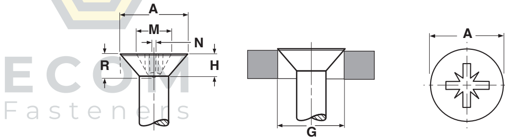
POZIDRIV® (TYPE 1A) FLAT HEADS FOR SELF-TAPPING SCREWS
