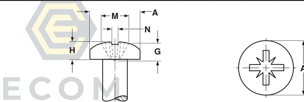
POZIDRIV® (TYPE 1A) PAN HEADS FOR SELF-TAPPING SCREWS
