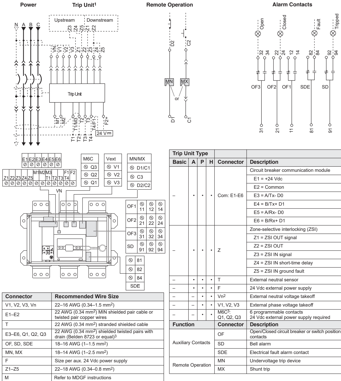
FIG. 3 : Accessory Control Wiring Diagram (English)
