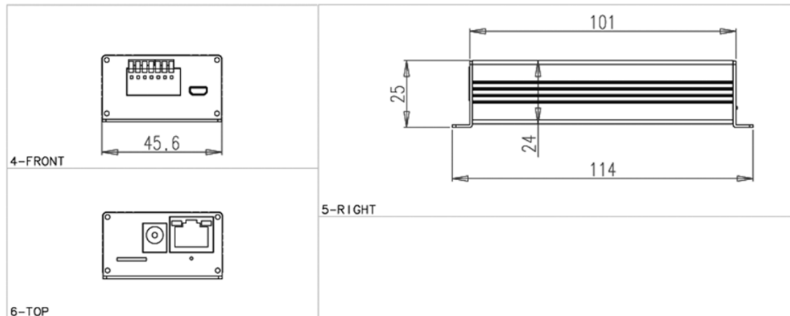
Figure 2-2. Dimensions
