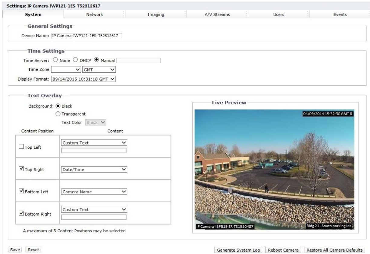
FIGURE 3-3: SYSTEM SETTINGS
