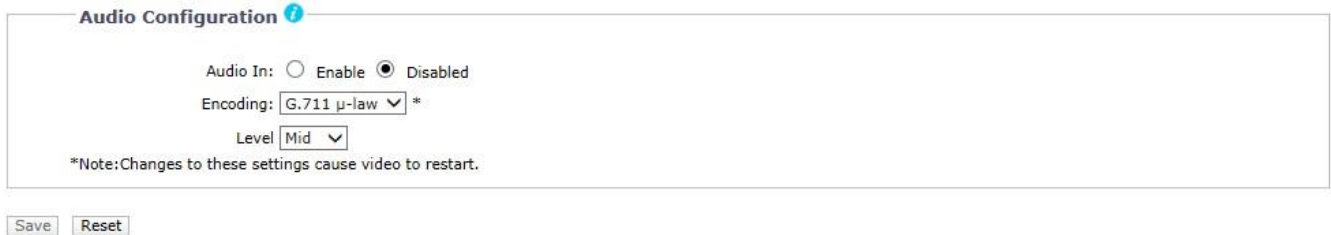
FIGURE 3-30: AUDIO CONFIGURATION
