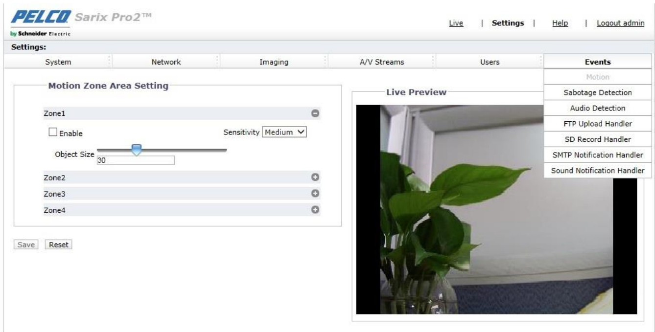
FIGURE 3-36: EVENTS SETTINGS
