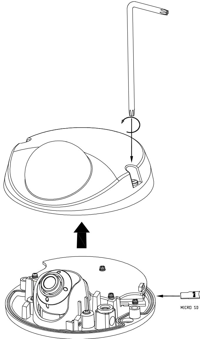
FIGURE 2 - 1: DISASSEMBLING THE CAMERA
