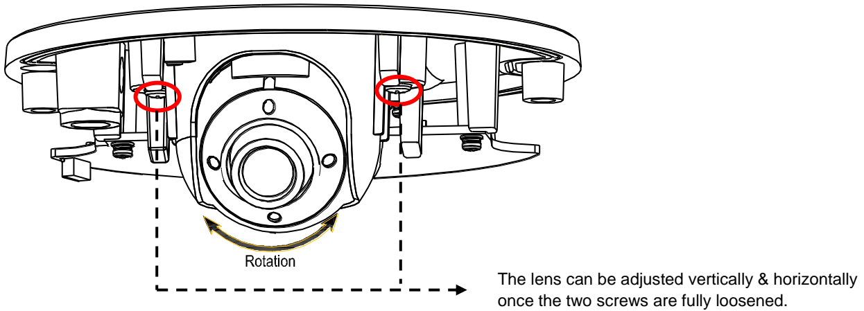
FIGURE 2 - 5: ADJUSTING THE FOCUS POSITION
