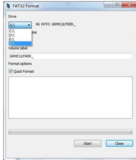
FIGURE 3-45: FAT32 FORMAT
