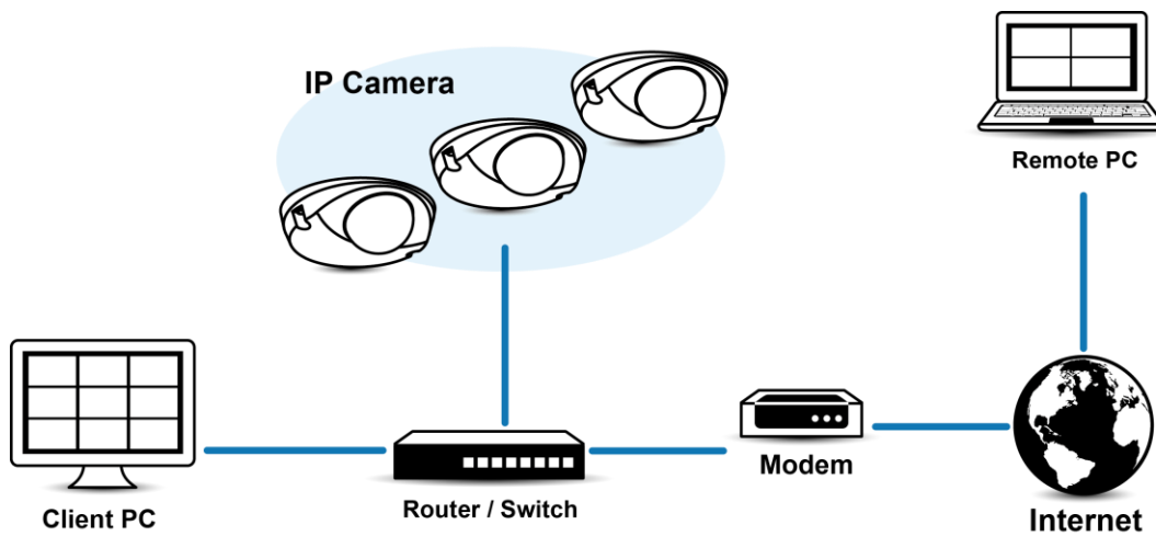
FIGURE 2 - 8: NETWORK TOPOLOGY
