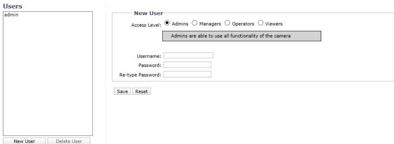
FIGURE 3-35: NEW USERS
