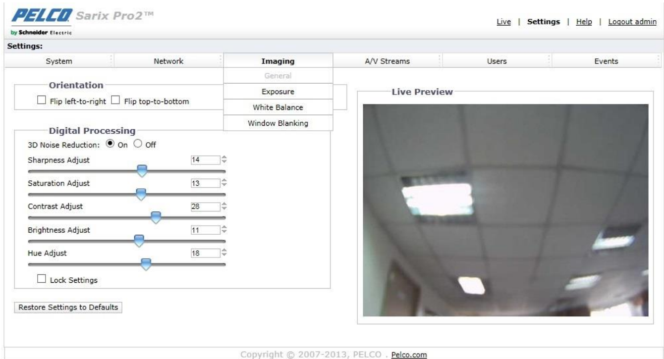
FIGURE 3-21: IMAGING SETTINGS
