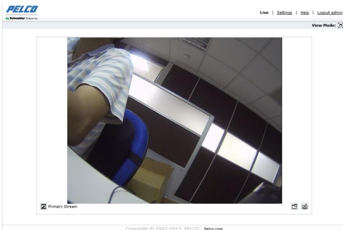
FIGURE 3-1: LIVE VIEW
