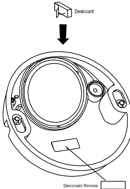
FIGURE 2 - 6: STICKING DESICCANT
