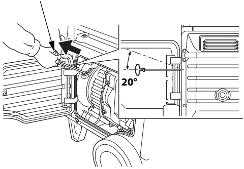
STARTER GRIP
