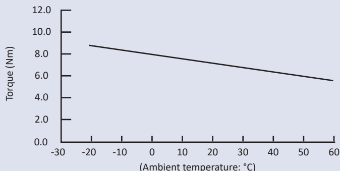
Temperature characteristics of FDN-63A-603 series (Rotation speed: 20 rpm)
