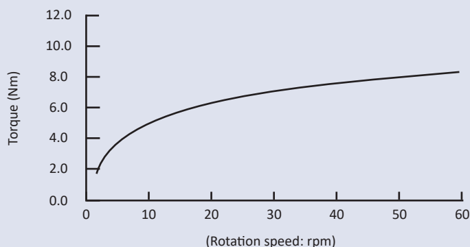
Speed characteristics of FDN-63A-603 series (Measurement temperature: 23°C)
