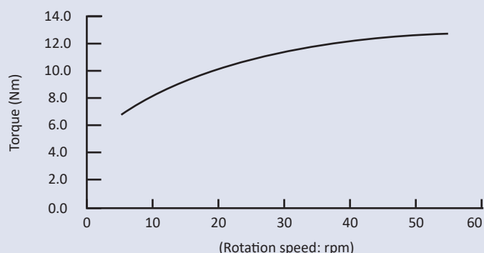
Speed characteristics of FDN-70A-114 series (Measurement temperature: 23°C)
