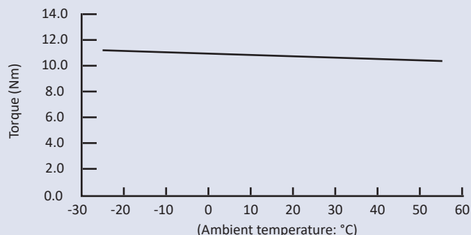
Temperature characteristics of FDN-70A-114 series (Rotation speed: 20 rpm)
