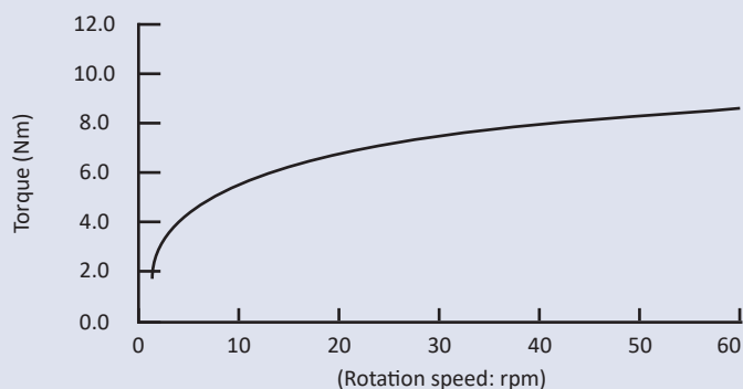
Speed characteristics of FDT-63A-703 series (Measurement temperature: 23°C)
