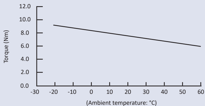
Temperature characteristics of FDT-63A-703 series (Rotation speed: 20 rpm)
