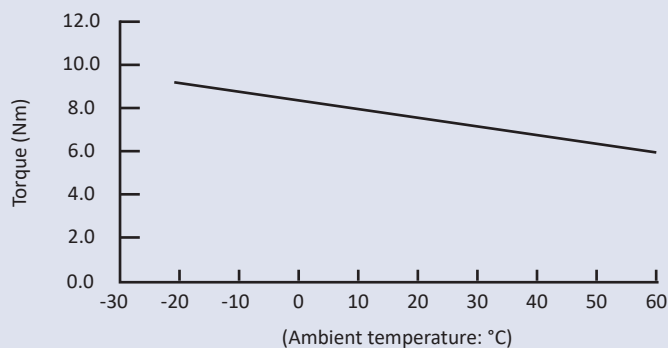
Temperature characteristics of FDT-63B-703 series (Rotation speed: 20 rpm)
