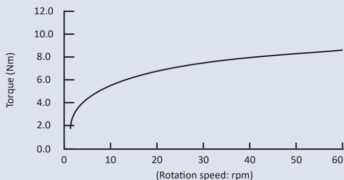
Speed characteristics of FDT-63B-703 series (Measurement temperature: 23°C)
