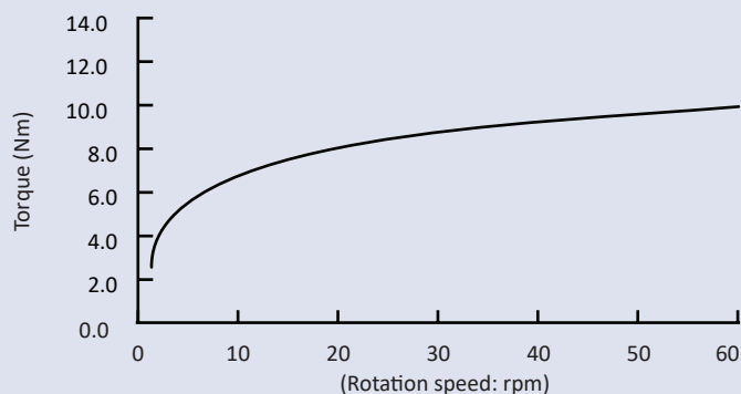
Speed characteristics of FDT-70B-903 series (Measurement temperature: 23°C)
