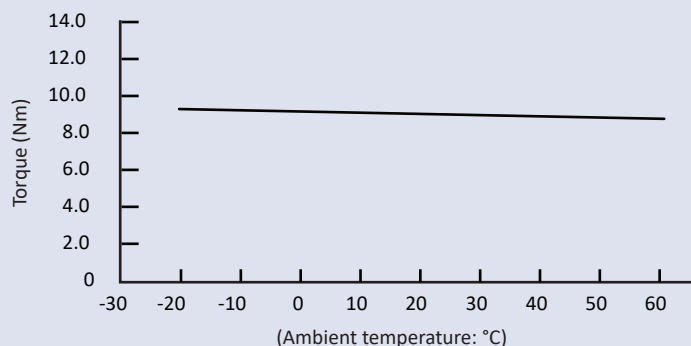
Temperature characteristics of FDT-70B-903 series (Rotation speed: 20 rpm)
