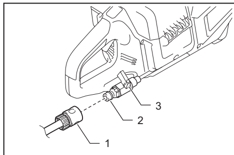
► 1. Coupling sleeve 2. Water inlet 3. Cock
