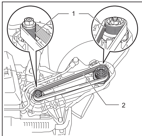
► 1. Rail on the pulley 2. Guide on the V-belt
