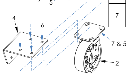
Casters and hardware kit
