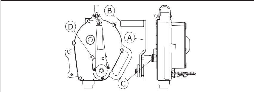
Figure 16 - SRD-R Inspection
