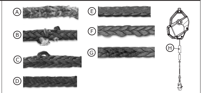
Figure 15 - Synthetic Rope Lifeline
