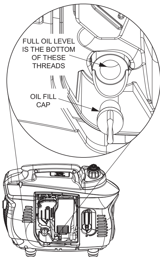
Figure 9 - Oil Fill
