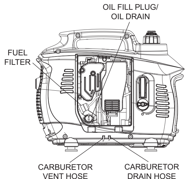
Figure 11 - Fuel Filter
