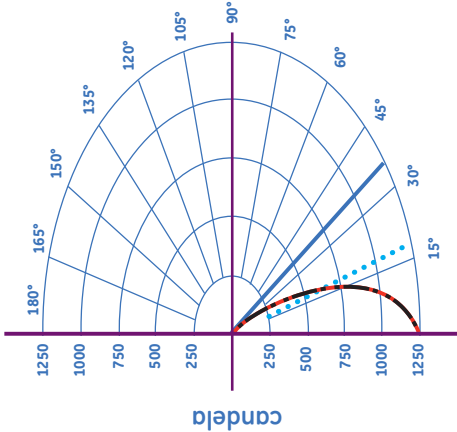
POLAR PLOT—40° BEAM
