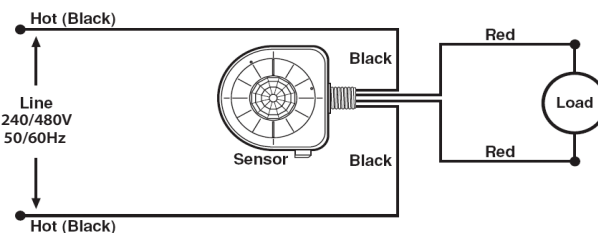
OSFHU (480V) Wiring Diagram
