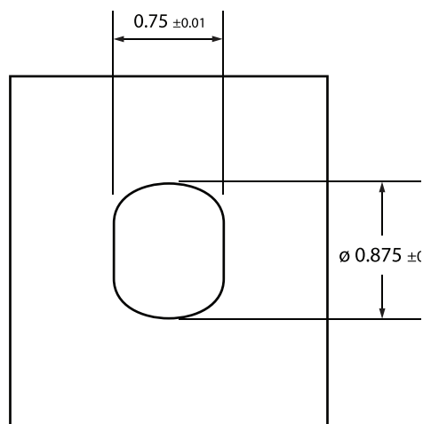
Sheet Metal* Punch Dimensions for Optional Snap-In Installation
