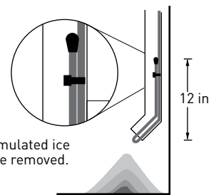
Figure 10. Heating cable in downspout
