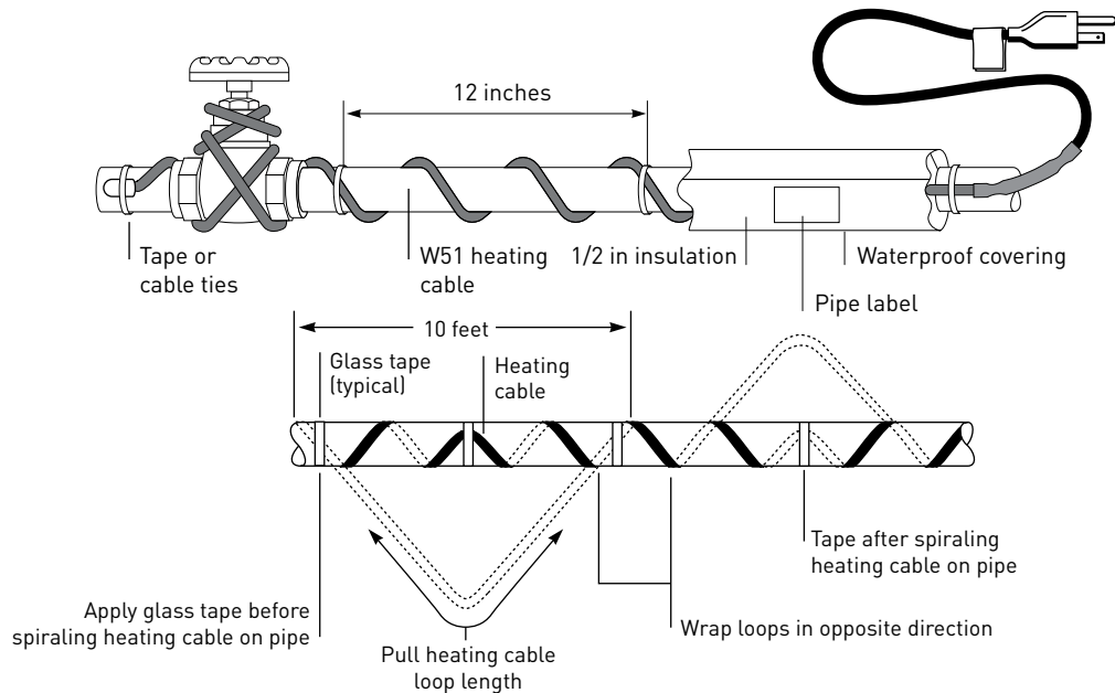
Figure 2. Spiral-traced installation
