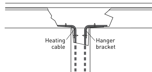
Figure 11. Hanger brackets
