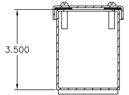
SECTION X-X Rotated 90 Degrees
