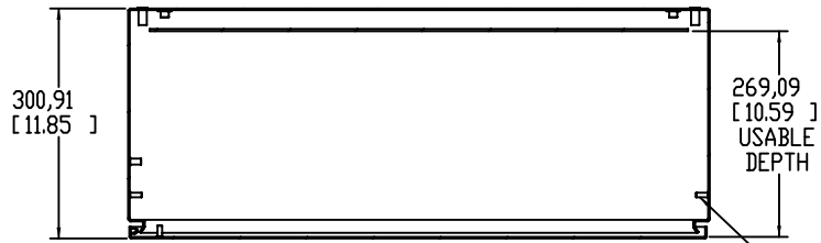
SECTION B-B
