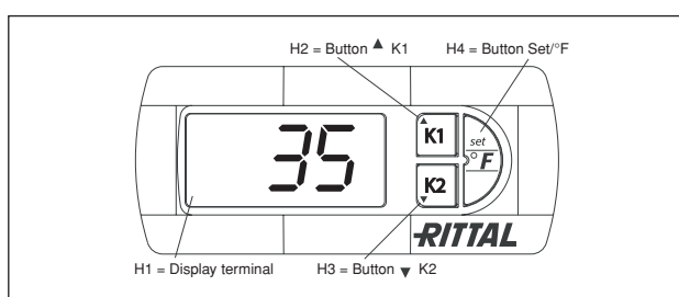
Fig. 6.1 Electronic control
