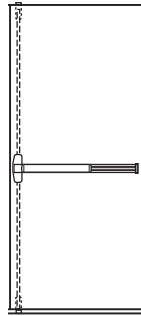
Concealed vertical rod (CVR)
