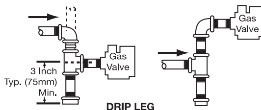
DRIP LEG
