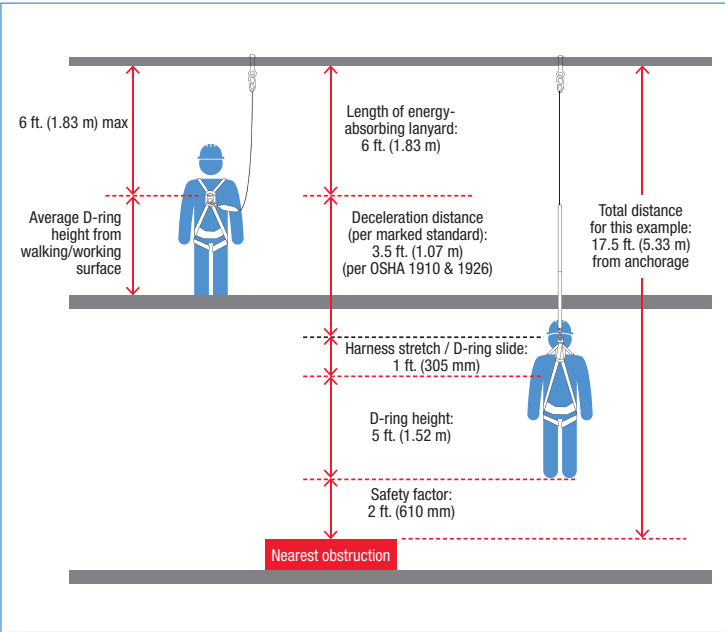
Figure 1 (Clearance)
